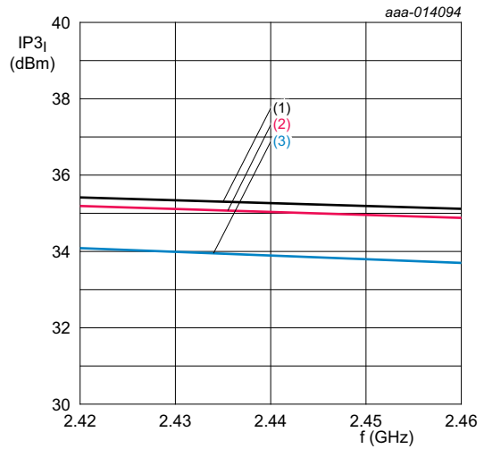
V_{CC} = 3.3\text{ V} ; V_{I(CTRL)} = 0\text{ V} ; two tone; 5 MHz spacing; P_i = 3\text{ dBm} ; bypass mode (1) T_{amb} = -40\text{ }^{\circ}\text{C} (2) T_{amb} = +25\text{ }^{\circ}\text{C} (3) T_{amb} = +85\text{ }^{\circ}\text{C}
